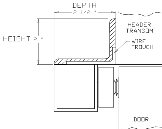
1194 ANGLE BRACKET
