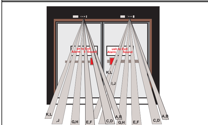
Figure 10: Masking a Dual Mount
