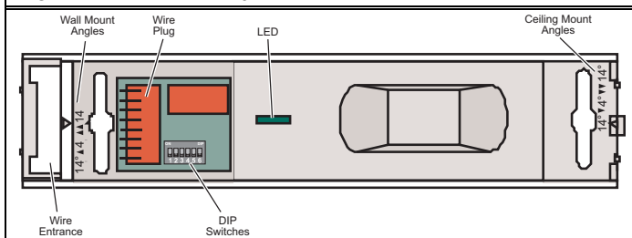
Figure 2: Location of Major Items
