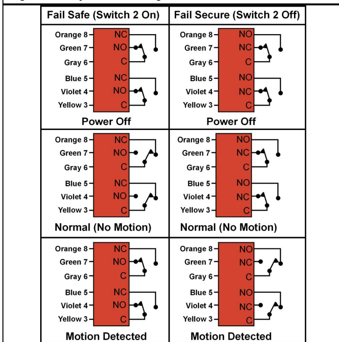
Figure 4: Relay Contact Wiring
