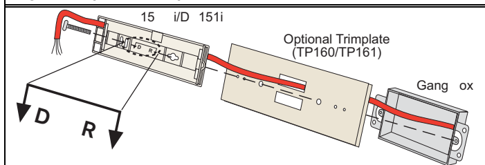
Figure 1: Optional Trimplate
