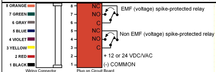
Figure 3: Connector to Plug Orientation (Default Switch Settings)
