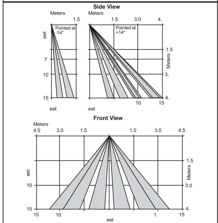
Figure 9: Standard Patterns for a Wall-mounted Unit
